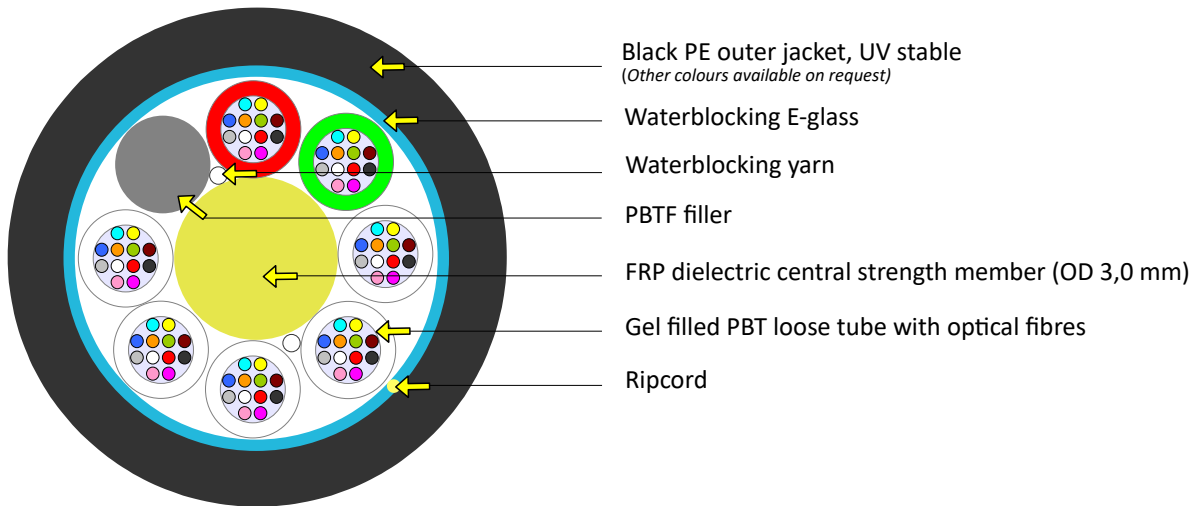
The picture represents a cable with 84 optical fibres.
