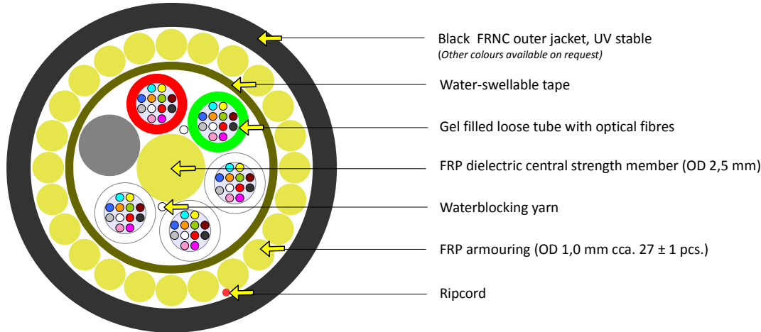
The picture represents a cable with 60 fibres
